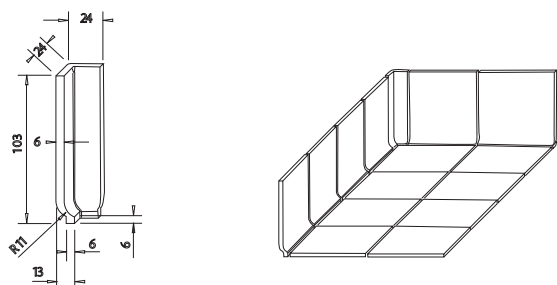
sokl vnitřní roh | skirting inside corner (GSIRCxxx)
